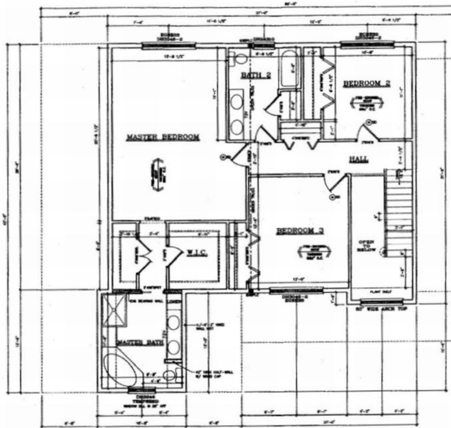
① SECOND FLOOR PLAN
