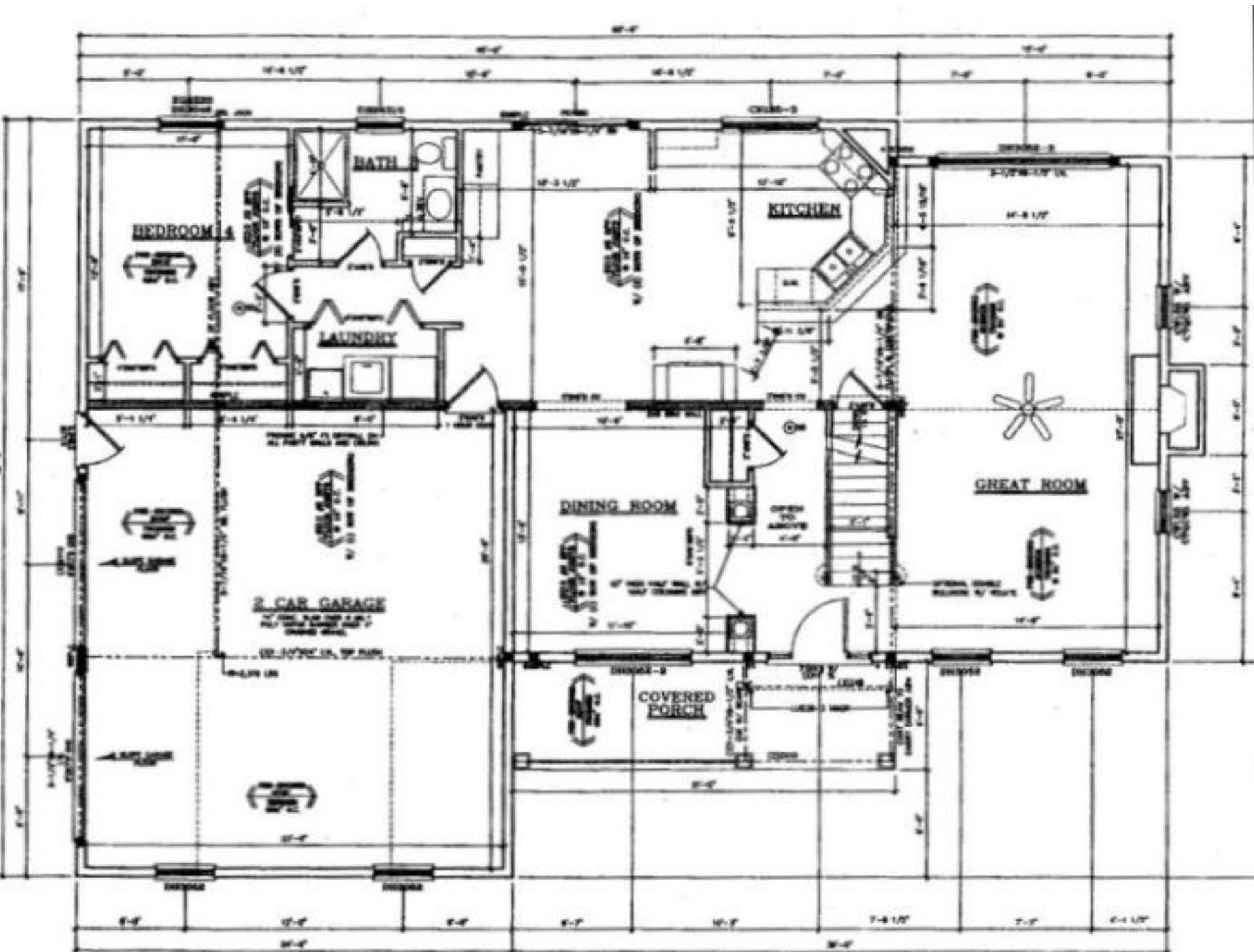
① FIRST FLOOR PLAN
